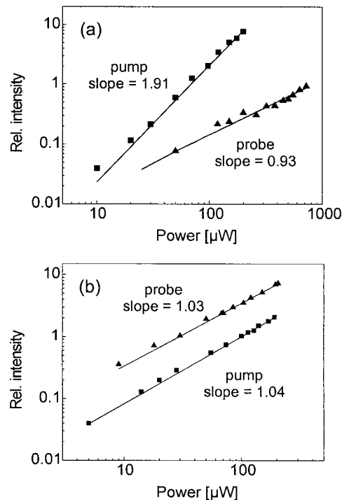
FIGURE 2 Logarithmic plot of the Kerr signal intensity as a function of incident beam powers. (a) Homodyne-detected optical Kerr effect signal; (b) Optically heterodyne-detected Kerr signal. ■, variations in the pump intensity; ▲, dependence of the signal on the probe beam intensity; —, least-square fits to the experimental data.
