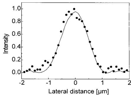
FIGURE 3 OHD Kerr signal measured (●) when scanning a 1- \mu\text{m} glass bead laterally through the focal volume of a 20 \times , 0.5 NA dry objective lens. —, CARS signal intensity as observed from the same bead.
