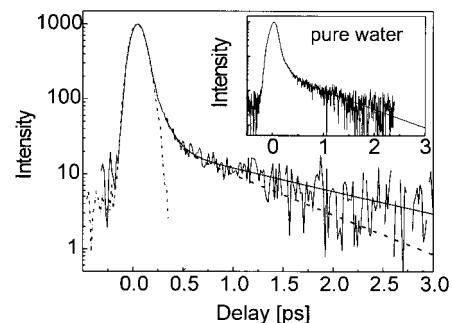
FIGURE 5 Intracellular optically heterodyne-detected OKE signal as a function of the delay between pump and probe. Single traces are recorded from different positions in the cell cytoplasm. The profile presented is the average of 100 individual measurements taken from five different cells. A least-square fitting procedure gives an exponential relaxation time \tau = 1.35 ps. The dotted line refers to the signal obtained from the supporting glass coverslip, 10 \mu\text{m} below the cells, and is indicative of the temporal resolution of the OKE experiment. The dashed line represents the fit to the response of pure water, also shown in the inset, with a relaxation constant of \tau = 0.79 ps.
